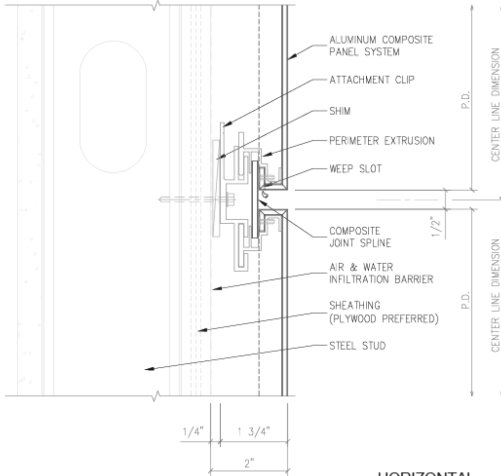
HORIZONTAL JOINT DETAIL
